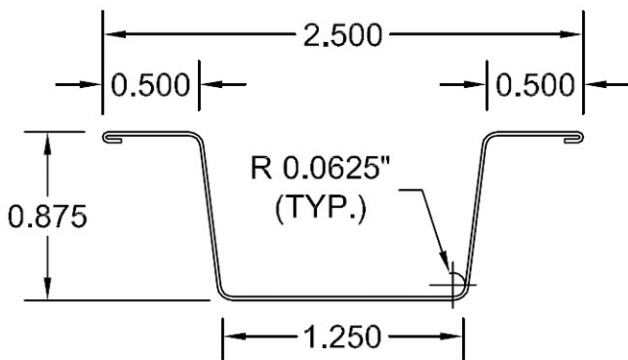
Light gauge (L.G.)
